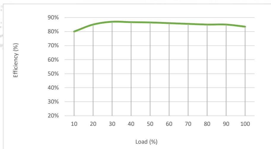
SDM02T0505, with nominal input voltage
