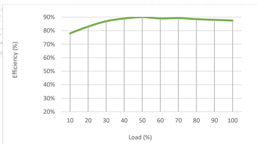
SDM02T1205, with nominal input voltage
