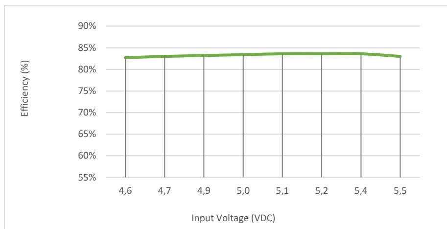
SDM02T0505, with full Load
