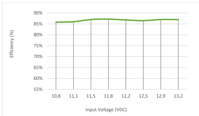
SDM02T1205, with full Load
